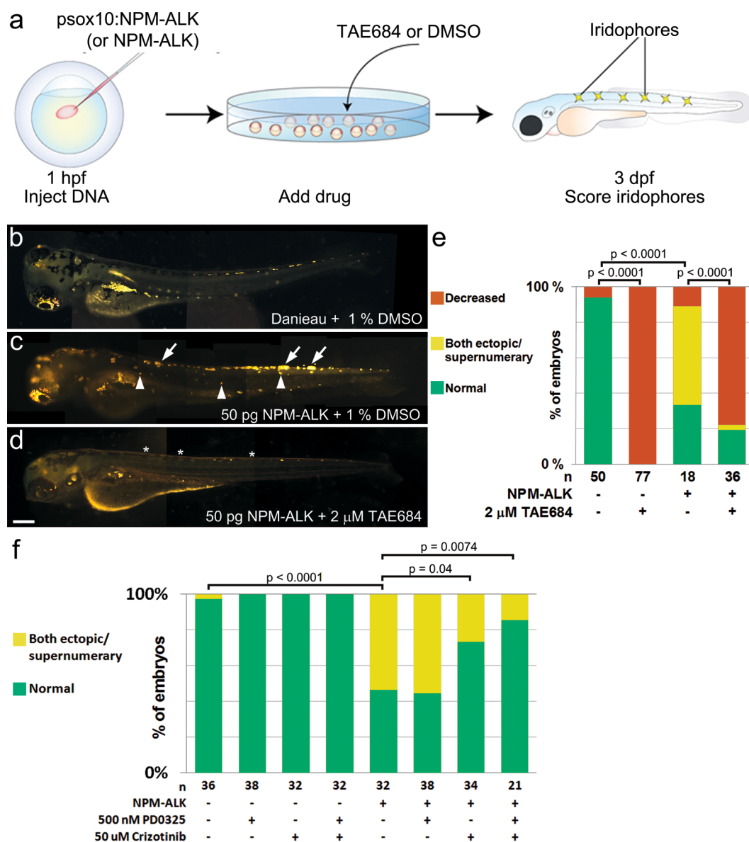
Figure 3. TAE684 inhibits NPM-ALK in vivo and reduces endogenous iridophores. Wild-type embryos were injected with 50 pg of psox10:NPM-ALK and treated with 2 \mu M TAE684 ALK inhibitor or DMSO control. (a) Schematic of experiment of this figure and Figure 4. (b–d) Incident light images at 3 dpf of control uninjected, nontreated embryo (b), NPM-ALK injected DMSO-treated sibling (c), and NPM-ALK injected TAE684-treated siblings (d). Injected embryos (c) have ectopic (arrowheads) and supernumerary (arrows) iridophores when compared to the uninjected control (b). Injected embryo treated with TAE684 has fewer iridophores than controls in eyes and trunk (asterisks) and no ectopic iridophores or large clusters (d). Ratios of embryos with normal, ectopic/supernumerary, and decreased iridophore numbers are quantitated in panel e. Differences between treatments are significant (Freeman–Halton extension of Fisher exact probability test; p values shown); numbers treated ( n ) in each category shown below each column. (f) Iridophore number in dorsal stripe position after treatment with Crizotinib and/or MEK inhibitor PD0325901 (PD0325). Comparisons assessed using Fisher's exact probability test. Note that Crizotinib treatment results in significant decrease in ectopic/supernumerary iridophore number compared with controls and that a low dose (500 nM) of PD0325901 (ineffective on its own) sensitizes the Crizotinib effect. Scale bar, 200 \mu m.
