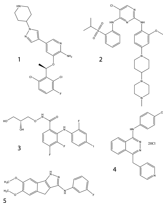
Figure 1. Structures of receptor tyrosine kinase inhibitors used in this study. [1] Crizotinib; [2] TAE684; [3], PD0325901; [4] Vatalanib; [5] PDGFR/Kit tyrosine kinase inhibitor IV.
