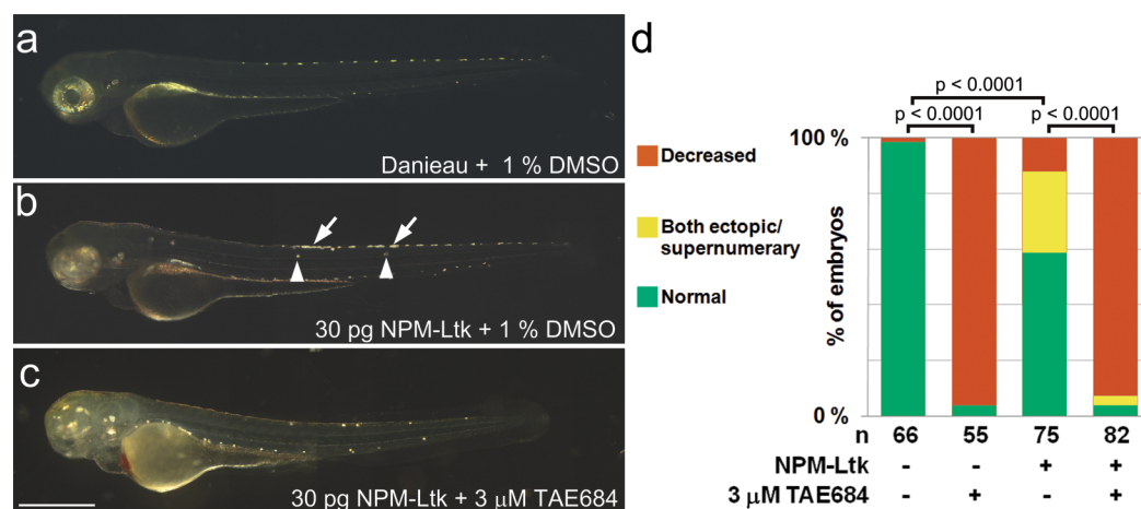
Figure 4. TAE684 inhibits NPM-Ltk. Wild-type embryos were injected with 30 pg of psox10:NPM-Ltk and treated with 3 \mu M of TAE684 (for schematic, see Figure 3). Incident light images (a–c) at 3 dpf of control uninjected, nontreated embryo (a); NPM-Ltk injected, DMSO-treated sibling (b); and NPM-Ltk injected TAE684-treated siblings (c). Injected embryos (b) have ectopic (arrowheads) and supernumerary iridophores (arrows) when compared to the uninjected control (a). Injected, TAE684-treated embryos have fewer iridophores than control in eyes and trunk and no ectopic iridophores or large clusters (c). Ratios of embryos with different phenotypes are quantitated in panel d, as in Figure 3e; differences between treatments are significant (Freeman–Halton extension of Fisher exact probability test; p values shown). Scale bar, 500 \mu m.
