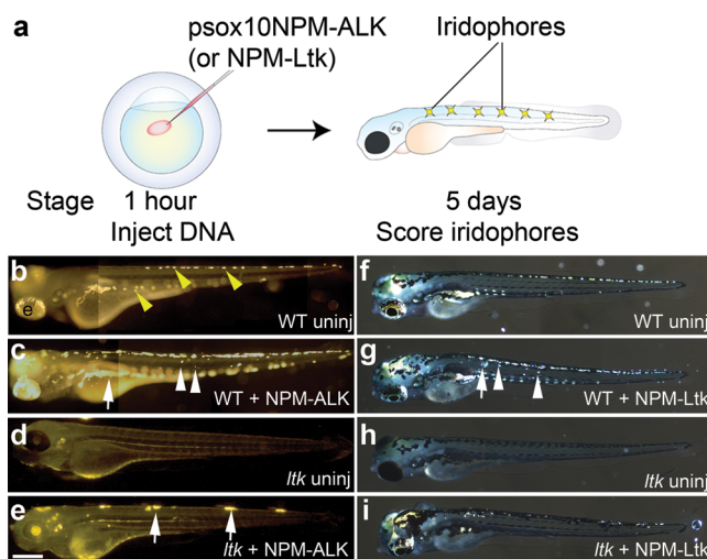
Figure 2. NPM-ALK and NPM-Ltk expression drives iridophore development. (a) Schematic of experiment. Note that the sox10 promoter fragment used in this construct has been shown to drive expression in neural crest, 20 so that these transiently transgenic embryos are expected to express the activated ALK or Ltk kinase in a tissue-specific, but mosaic, manner. (b–e) Injection of 230 pg of psox10:NPM-ALK into wild-type (c) or ltk ty82 mutants (e) increases iridophore numbers compared with uninjected controls (b,d). Iridophores are the prominent silver–gold spots, seen either as individual cells (yellow arrowheads in b) or as clusters (e.g., on surface of eye (e) in panel b). In wild-types, expression generates supernumerary (arrows) and ectopic (arrowheads) iridophores, whereas in ltk mutants, iridophore development is rescued, often forming large clusters (arrows). (f–i) Analogous experiment using psox10:NPM-Ltk gave very similar phenotypes. All fish photographed at 5 dpf. NB fish in panels b–e have been treated with phenylthiourea and hence lack melanin. Here, and in all subsequent figures, embryos are shown dorsal up and anterior to the left. Scale bar, 200 μm.
